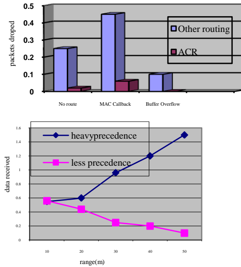
Figure2. Comparison of high precedence node dropping in ACR & other routing techniques Figure3. Analysis of high precedence nodes received ACR & MACR
