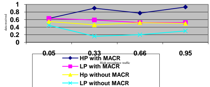
Figure4. Analysis of High precedence nodes received in high traffic
