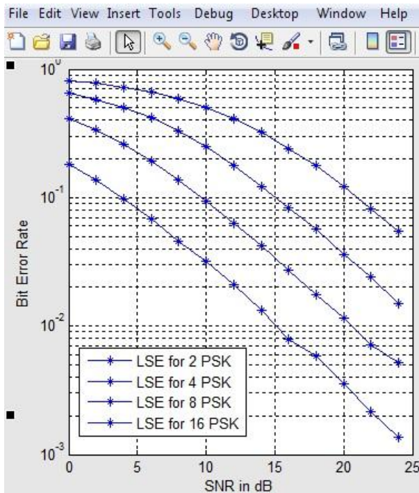
Fig 3: PSK in LSE graph for bit error rate of proposed work, implemented in Matlab.
