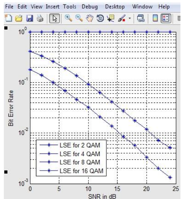
Fig 4: QAM in LSE graph for bit error rate of proposed work, implemented in Matlab.
