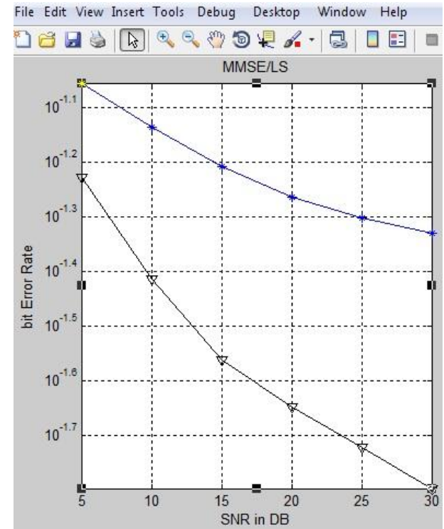
Fig 2: MMSE/LS graph for bit error rate of previous work, implemented in Matlab.
