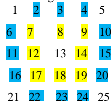
Fig.8 Network Neighborhood
