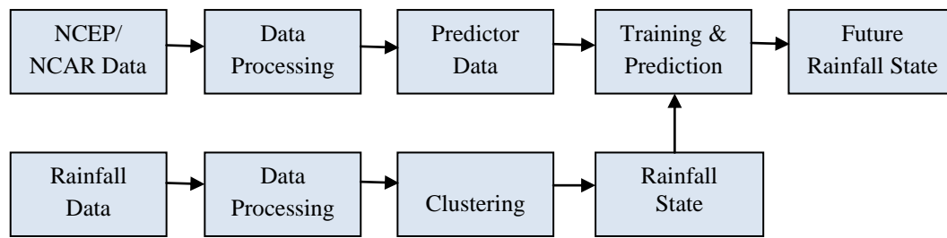
Fig 1: System Architecture
