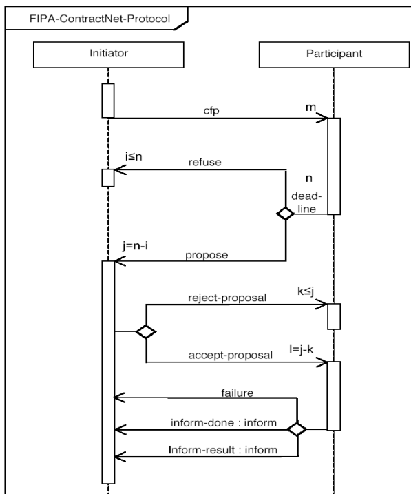
Fig 1: FIPA Contract Net Interaction Protocol
