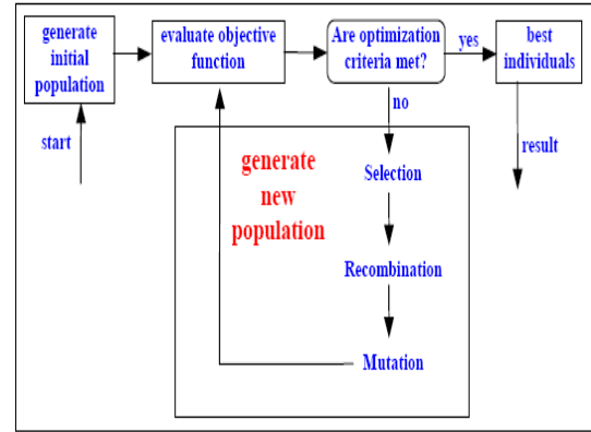
Fig 6: Structure of a single population Genetic algorithm
