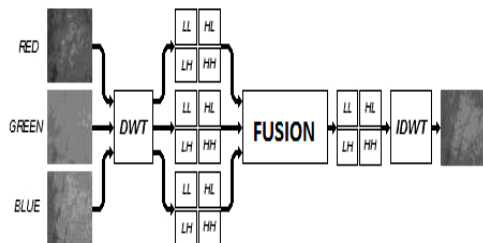
Fig 3: Multispectral image level fusion of Blue, Green and Red palmprint images
