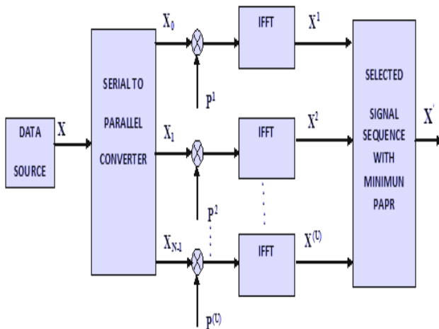
Fig. 1: Block diagram of the SLM scheme
