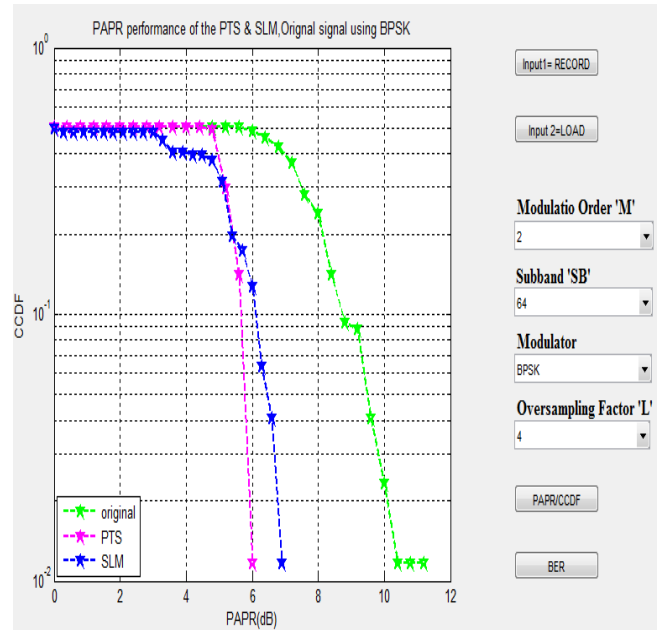
Fig. 7: CCDF vs. PAPR curve of PTS, SLM and Original while using BPSK modulator.
