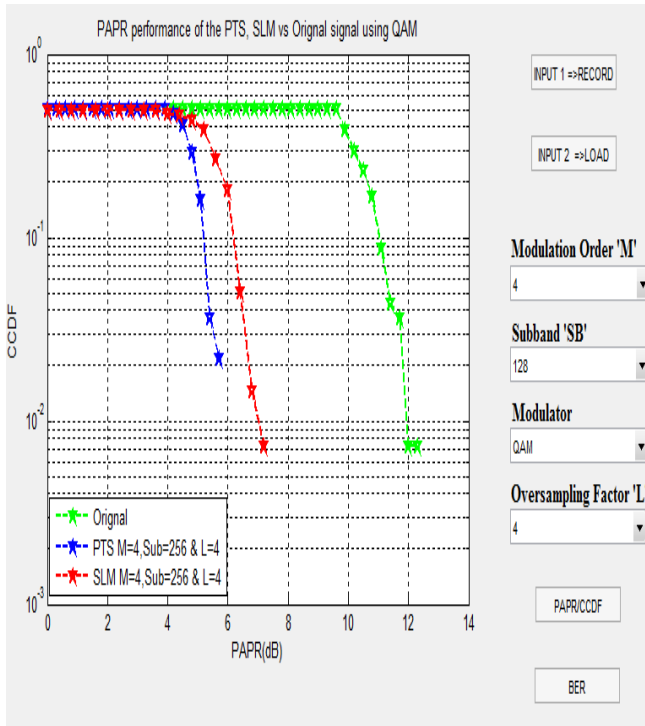
Fig. 4: CCDF/PAPR curve of Original, SLM & PTS schemes, while using QAM modulator.
