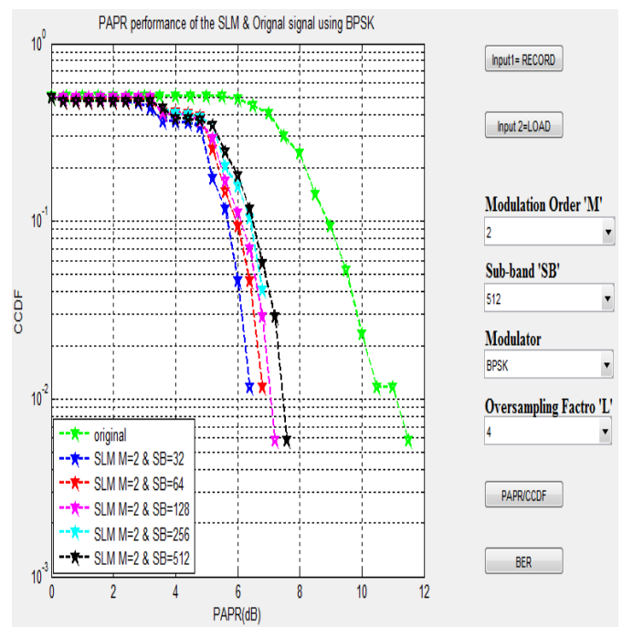
Fig. 8: CCDF vs. PAPR curve of Original, SLM schemes, while using BPSK modulator at various sub-bands.
