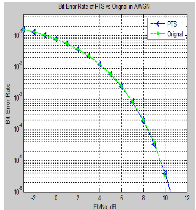
Fig. 10: BER curve of PTS & Original transmitted signal, while using QAM modulator.
