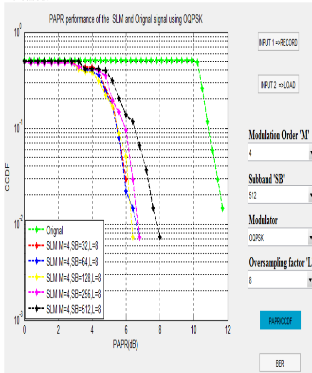
Fig. 6: CCDF vs. PAPR curve of Original, SLM schemes, while using OQPSK modulator at various sub-bands.
