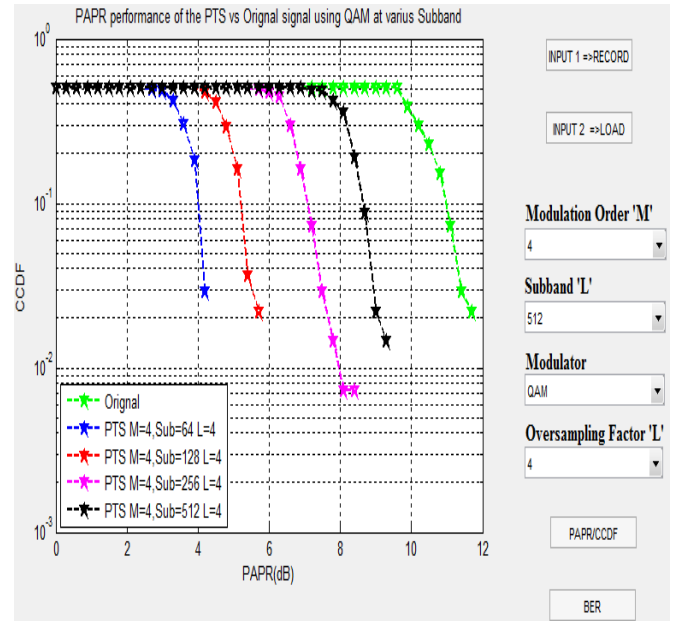
Fig. 5: CCDF/PAPR curve of Original & PTS schemes, while using QAM modulator at various sub-bands.
