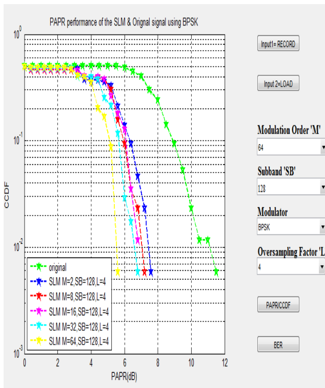
Fig. 9: CCDF vs. PAPR curve of Original, SLM schemes, while using BPSK modulator at various Modulation order.
