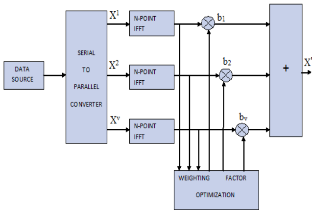
Fig. 2: Block diagram of partial transmit sequence scheme.
