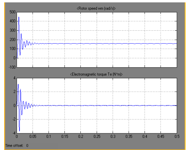
Figure 7. Motor speed and Torque
