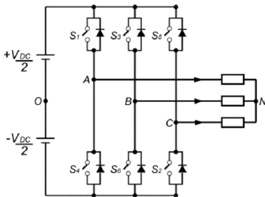
Figure 2. Three phase inverter configuration
