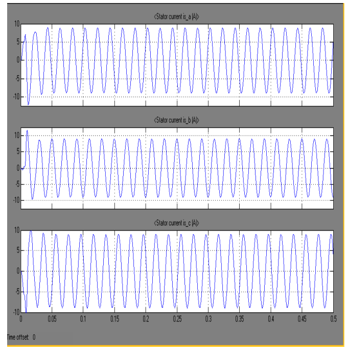
Figure 6. Motor Current results
