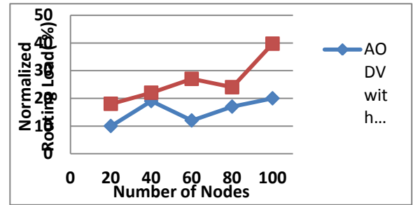
Fig. 4: Normalized Routing Load of AODV with and without malicious attack
