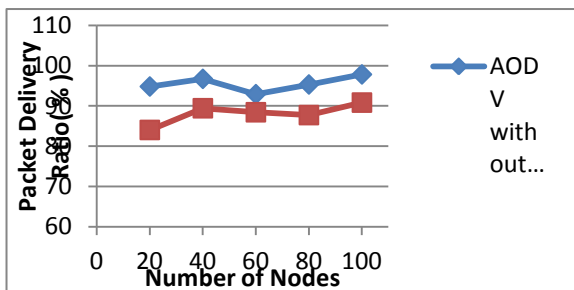
Fig. 2: Packet Delivery Ratio of AODV with and without malicious attack
