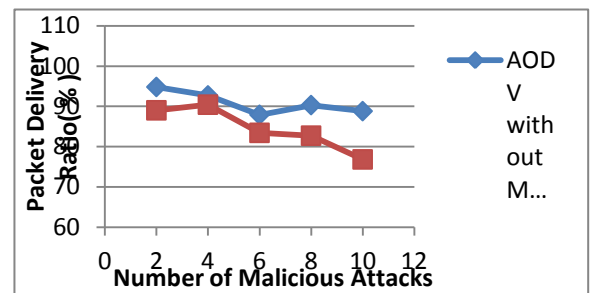
Fig. 5: Packet Delivery Ratio of AODV under Number of malicious attack
