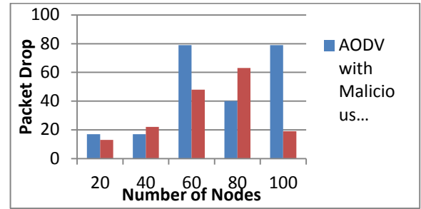
Fig. 3: Packet Drop of AODV with and without malicious attack
