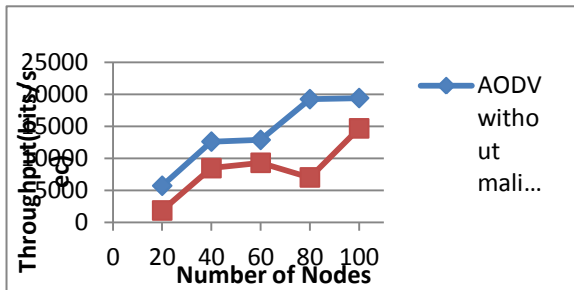
Fig. 1: Throughput of AODV with and without malicious attack
