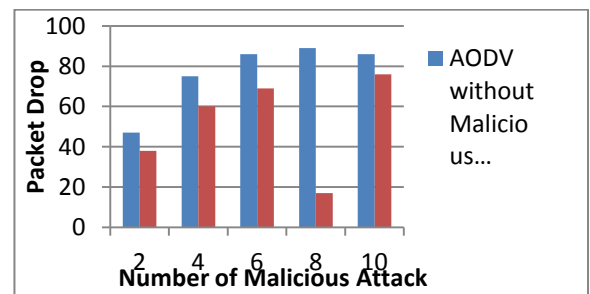
Fig. 6: Packet Drop of AODV under Number of malicious attack
