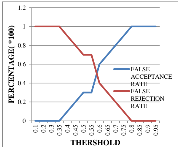
Figure 10: Dependence of False Acceptance Rate and False Rejection Rate on threshold
