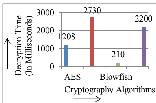
Fig. 4: Decryption time of Encryption Algorithms
