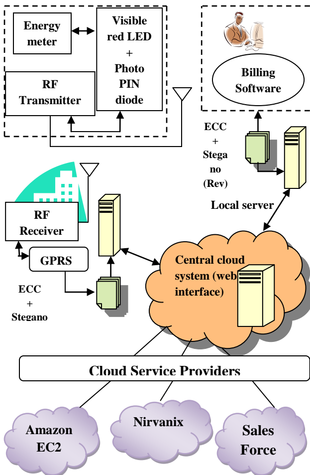
Fig.1 Proposed model of the entire system
