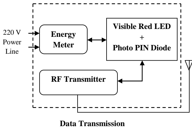
Fig.4: Additional H/W components interfaced with existing energy meter
