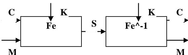
Fig.2 Steganography Process
