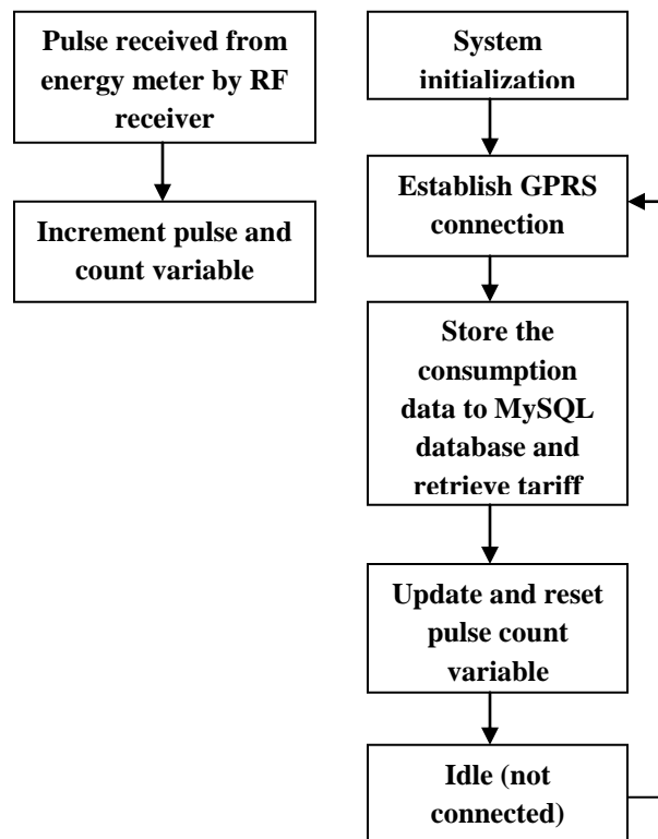
Fig.3 Flow diagram of System
