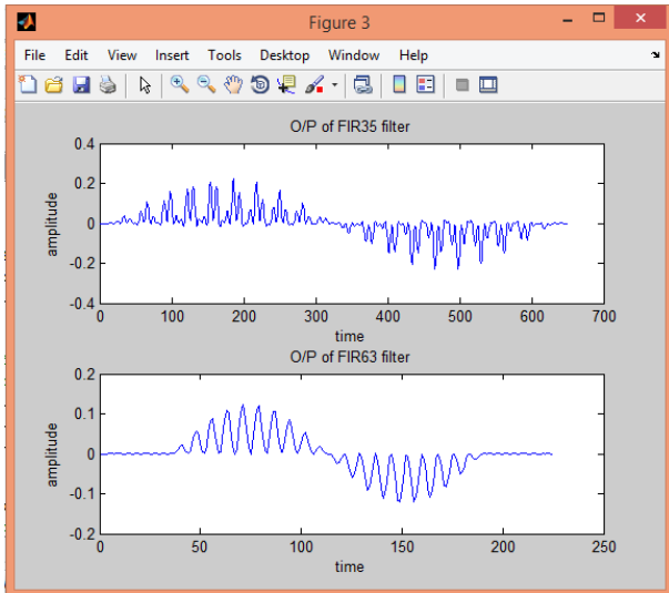
Fig. 6: Output of 35 tap and 63 tap filtering respectively
