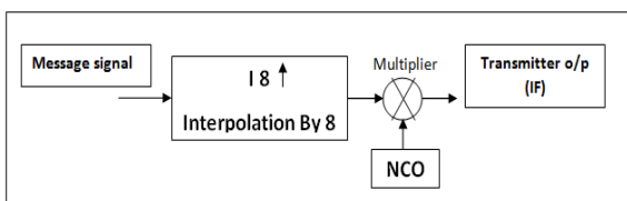
Fig. 3: Block diagram of transmitter
