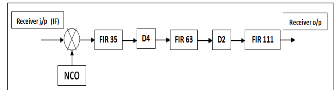
Fig. 4: Architectural block diagram of DDC at the receiver
