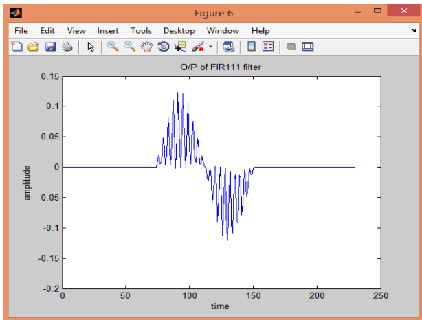
Fig. 7: Output of 111 tap FIR filter
