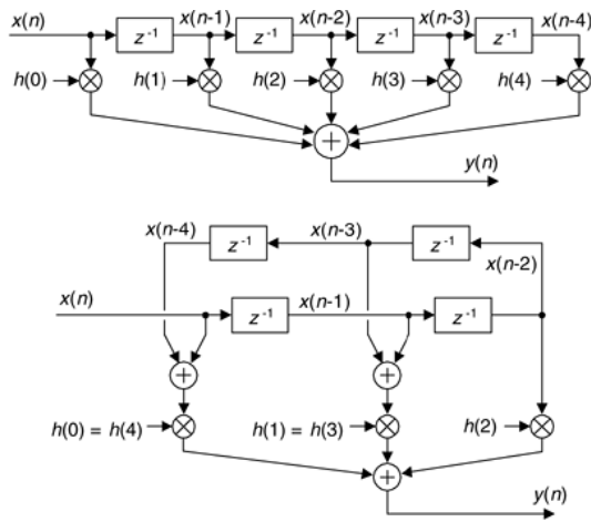
Fig. 2: Unfolded and Folded FIR structure
