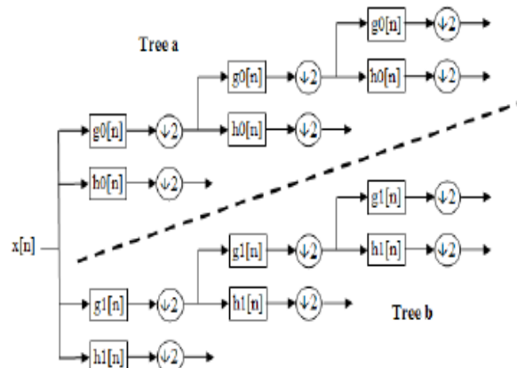
Fig.2 Structure of DT-CWT
