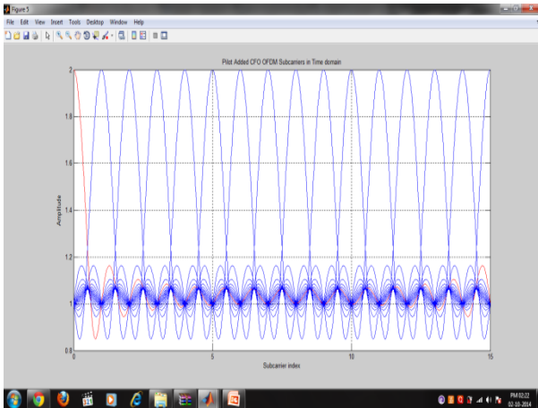
Figure 3:- Pilot added OFDM estimation
