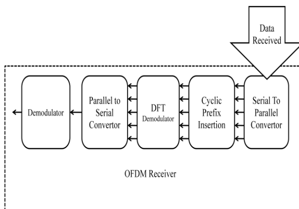
Figure 2 Receiver of OFDM
