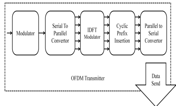
Figure 1 Transmitter for OFDM
