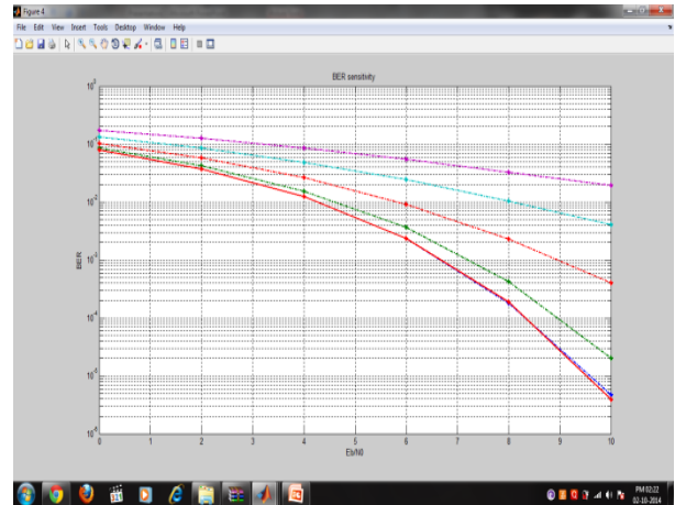
Figure 5: Comparison of BER Sensitivity
