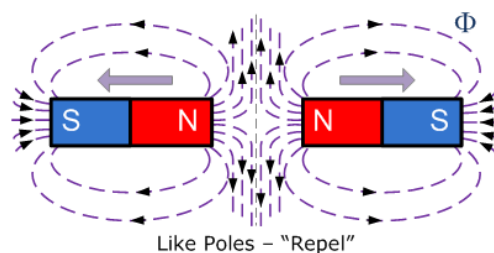
Figure 2: Like Poles Repel
