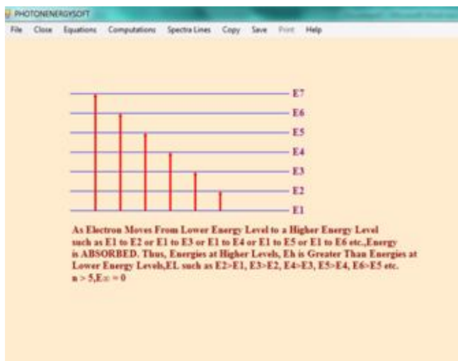
Figure 3: Absorption Spectral Lines; arrows pointing upward, indicating transition from lower energy level to higher energy level
