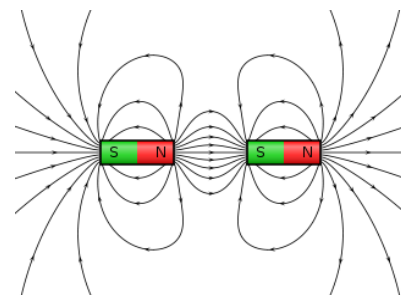
Figure 1: Unlike Poles Attract
