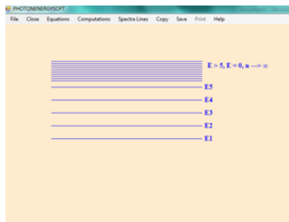
Figure 5: Compressed Spectral lines when E > 5
