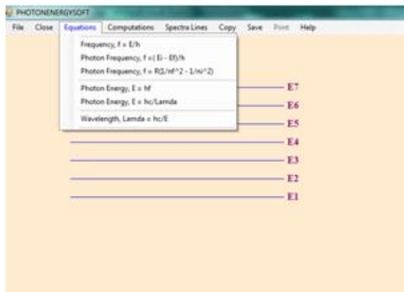
Figure 1: Labelled Energy levels, orbital No not shown
