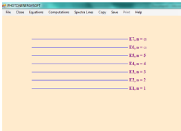
Figure 2: Labelled Energy levels, orbital No not shown
