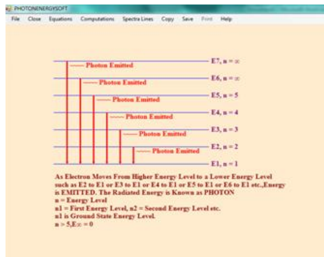
Figure 4: Emission of Photon; arrows pointing downward, indicating transition from higher energy level to lower energy level
