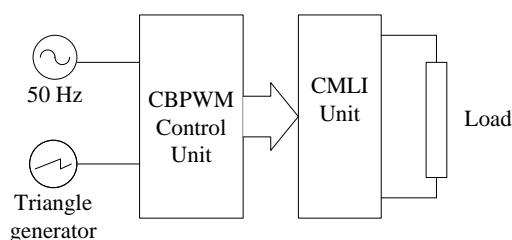
Fig. 5 System configuration
