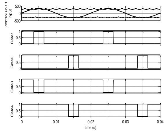
Fig. 11 Control unit 1 signal
