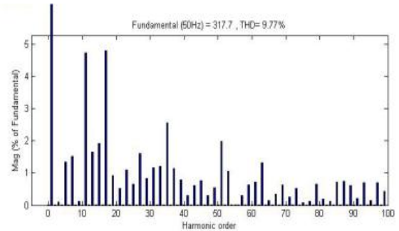
Fig. 18 Voltage frequency spectrum using carrier 500 Hz
