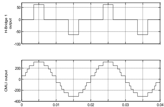
Fig. 12 H-Bridge 1 output and CMLI output
