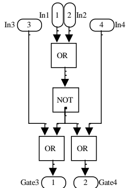
Fig. 10 Zero gate control
