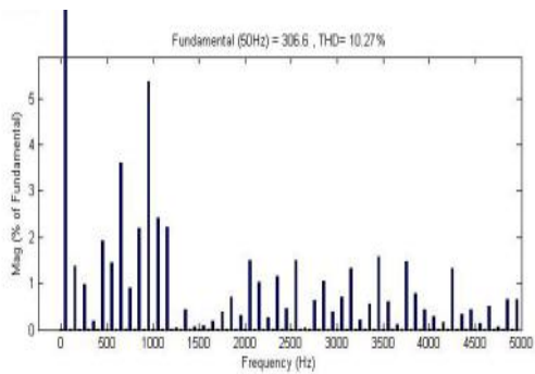
Fig. 16 Voltage frequency spectrum using carrier 1000 Hz
