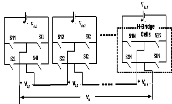
Fig. 1 Single-phase cascaded multilevel inverter
