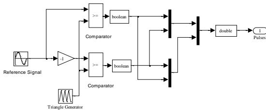
Fig. 9 Gate trigger generator
