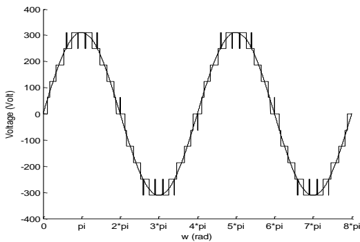
Fig. 15 CMLI output using carrier 1000 Hz
