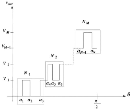
Fig. 4 Voltage output waveform
