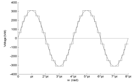
Fig. 17 CMLI output using carrier 500 Hz
