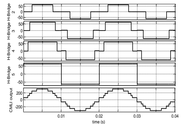
Fig. 13 H-Bridge 2-5 output and CMLI output
