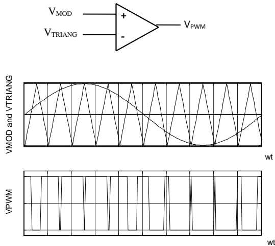
Fig. 2 Basic principle of PWM
