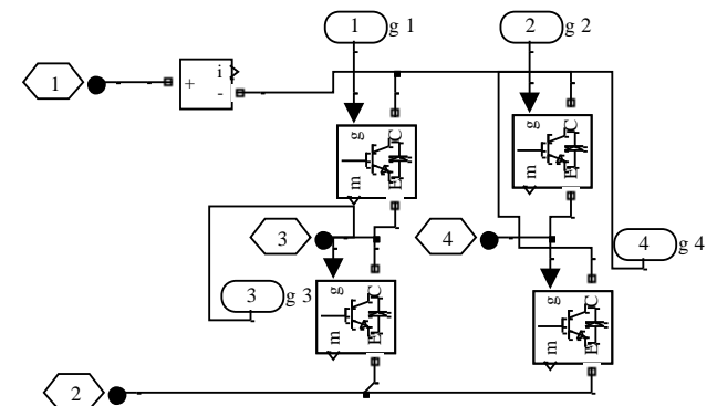
Fig. 7 H-Bridge circuit (INV1-INV5)
