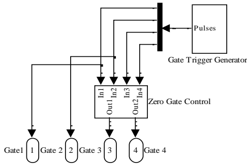
Fig. 8 Control unit circuit
