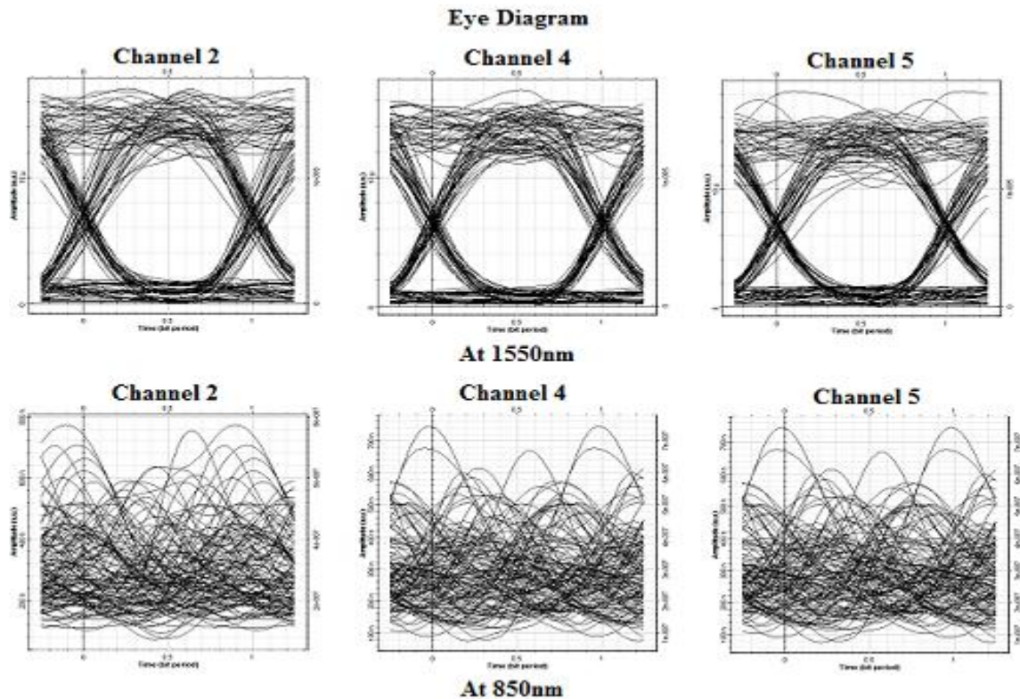
Fig 5: Eye Diagram at receiver pointing error of 3 \mu rad
