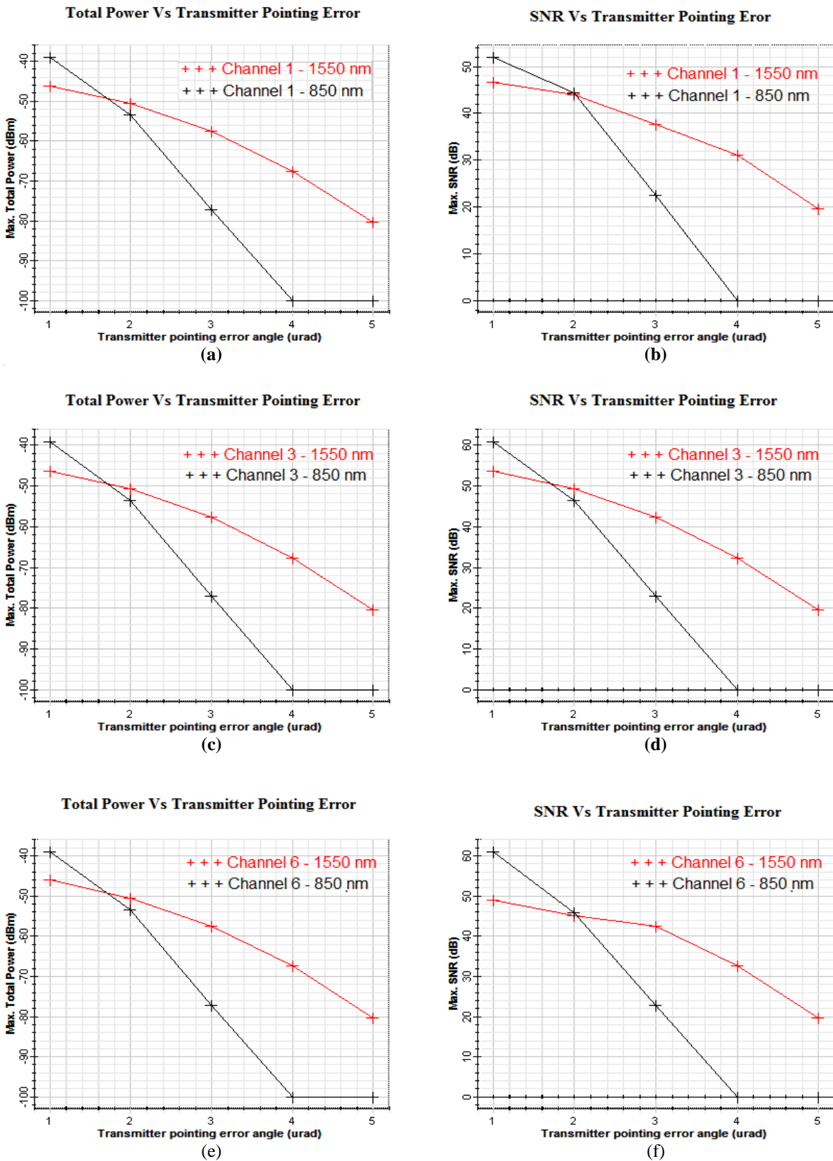
Fig 2: Total Received Power and SNR Vs Transmitter Pointing Error for (a & b) Channel 1 (c & d) Channel 3 (e & f) Channel 6
