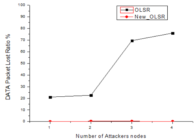
Fig 6: DATA packet Lost ratio VS Number of attacker nodes
