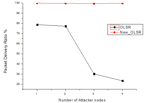
Fig 5: Packet Delivery Ratio VS Number of attacker nodes.
