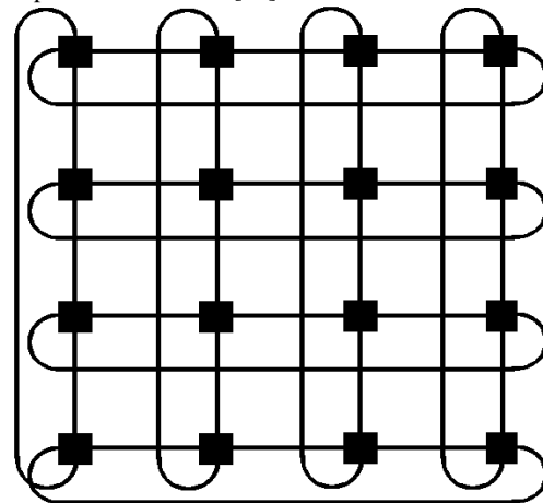
Fig 2: Torus network Source: Ville Rantala et al. “Network on Chip Routing Algorithm”
