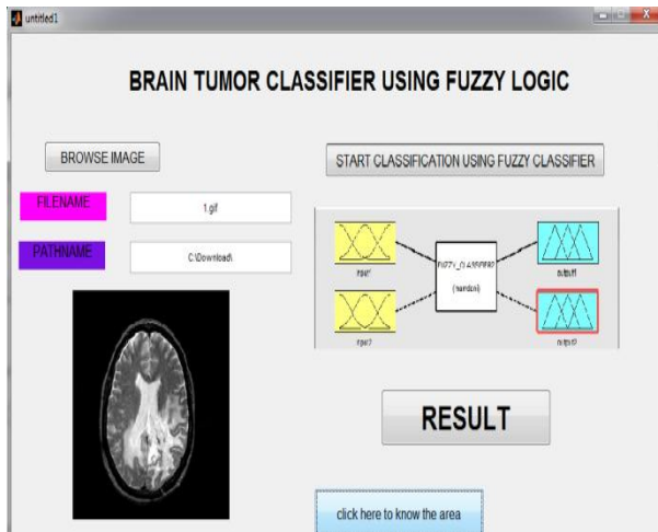
Fig 4.1: Take Input
