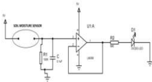
Fig 4 Circuit diagram of soil moisture sensor
