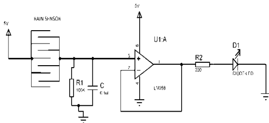
Fig 5: Circuit diagram of rain sensor
