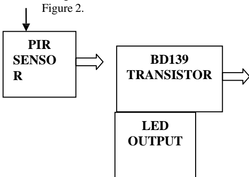
Fig 2: Block diagram of PIR sensor
