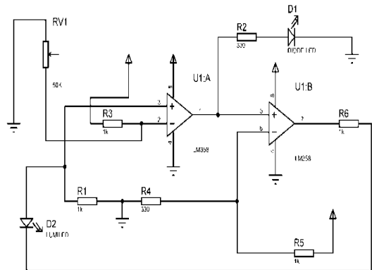
Fig 3: Circuit design of automatic lights on/off using photo diode
