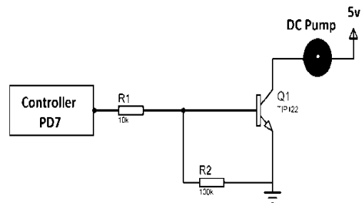
Fig 6: Circuit diagram of DC pump
