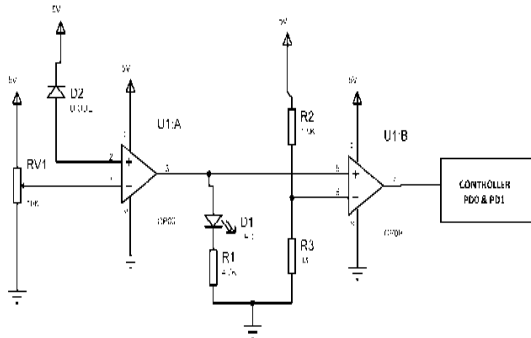
Fig 8: Receiver part of IR sensor
