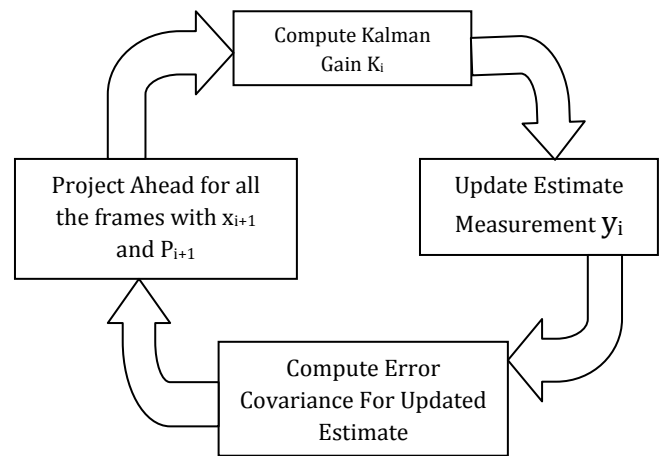
Fig.1 Frame by Frame Working of Kalman Filter
