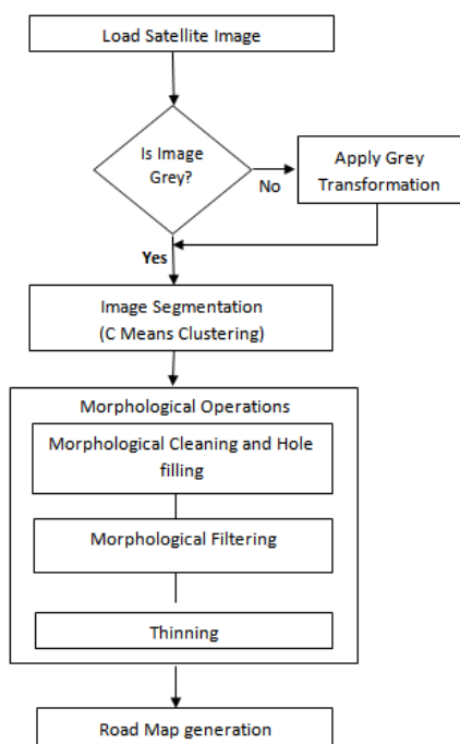
Fig 1: Flow chart of road network extraction
