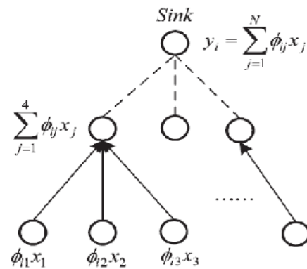
Fig.1. Data collection with the pure CS method in the tree structure
