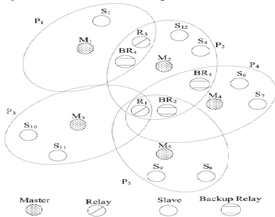
Fig 2: Scatternet after applying DRM
