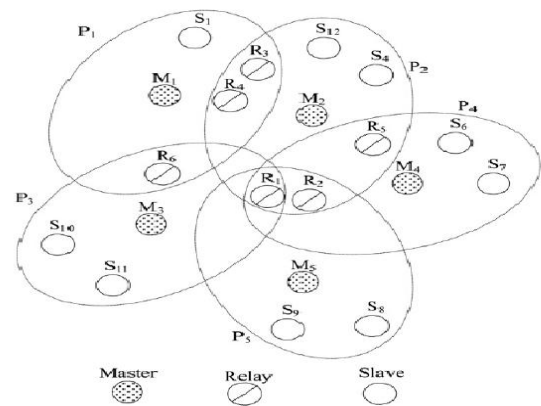
Fig 1: Illustration of Scatternet
