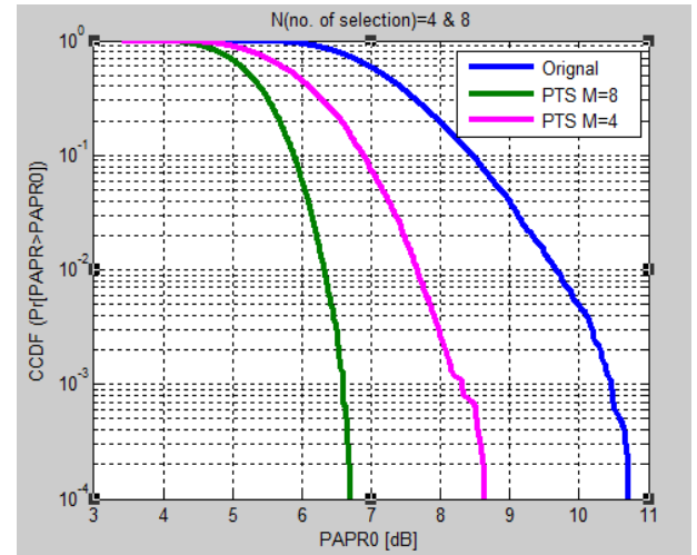
Figure 5. CCDFs of PAPR of PTS technique for M = 4 and 8 phase factors
