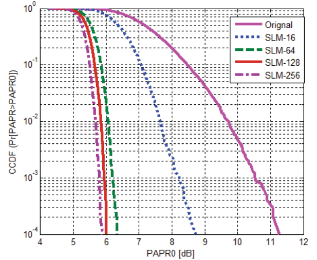
Figure 2. CCDFs of PAPR of SLM technique for N = 16, 64, 128 and 256 subcarriers
