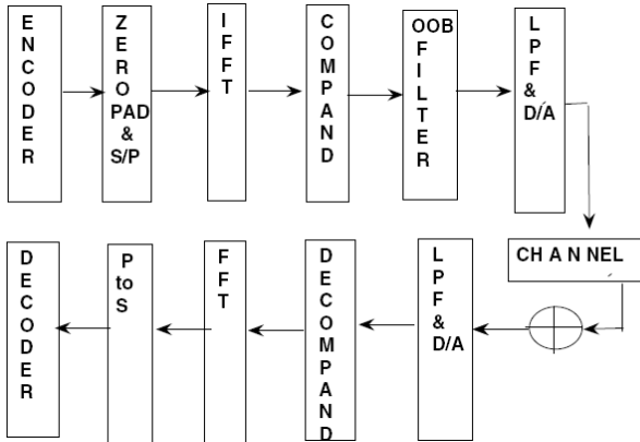
Figure 6. OFDM system using companding Technique[15]
