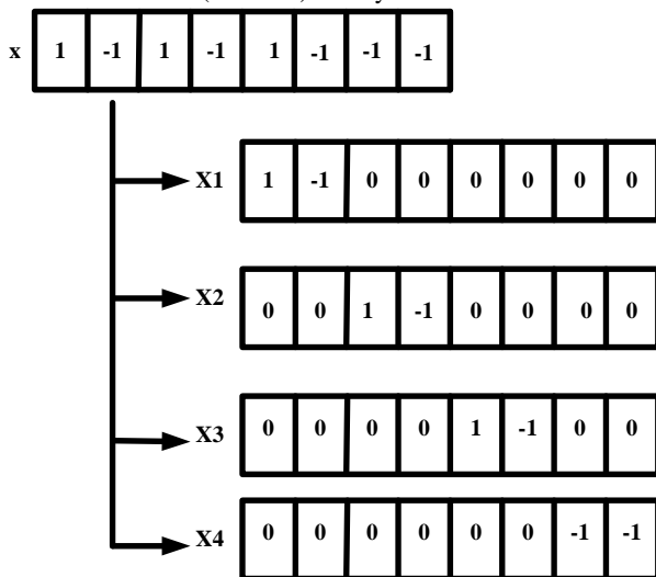
Figure 4. An example of adjacent subblock partitioning in PTS
