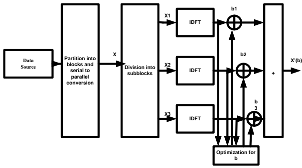
Figure 3. Block diagram of PTS scheme [7].
