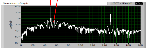
Fig 8: Winding Fault machine (50% winding faulted)
