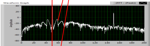
Fig 7: Winding Fault machine (20% winding faulted)
