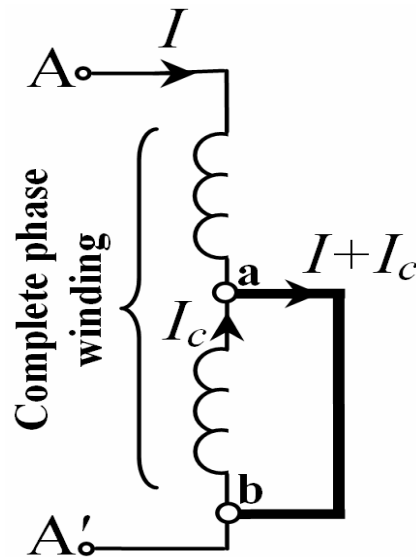
Fig 15: Short circuit Model
