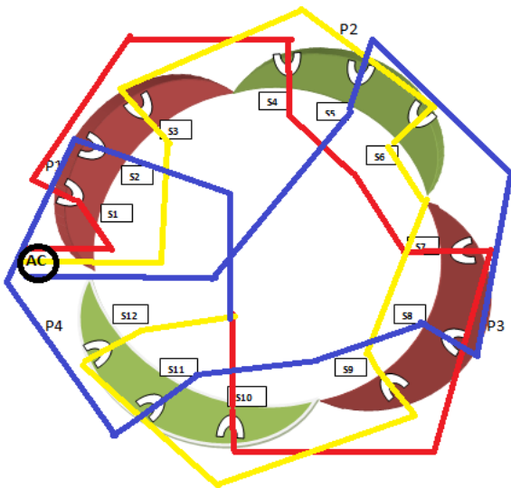
Fig 1: Stator winding
