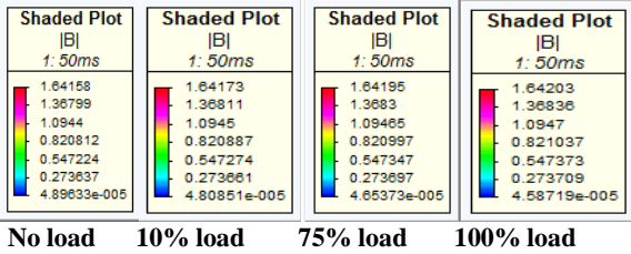
Fig 18: Flux Magnitude for less number of turns short circuited
