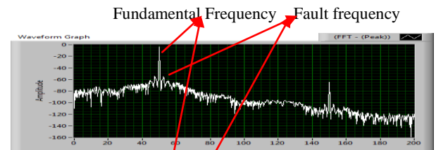
Fig 11: Winding Fault machine (1% winding faulted)
