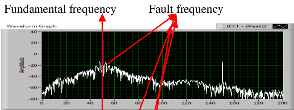
Fig 5: Winding Fault machine (1% winding faulted)
