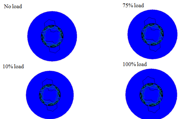
Fig 17: Flux Pattern for Healthy Machine at different load conditions
