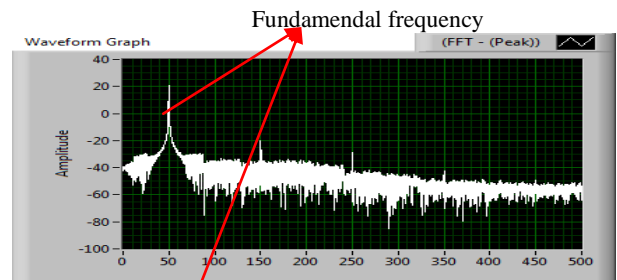
Fig 3: Healthy machine with no load
