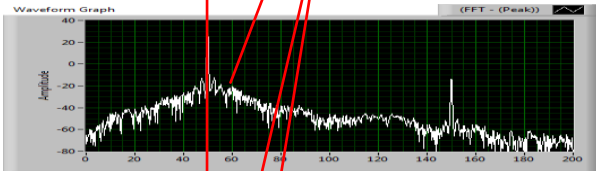
Fig 6: Winding Fault machine (2% winding faulted)
