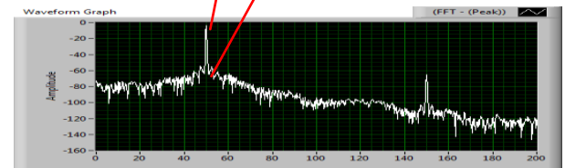
Fig 12: Winding Fault machine (2% winding faulted)
