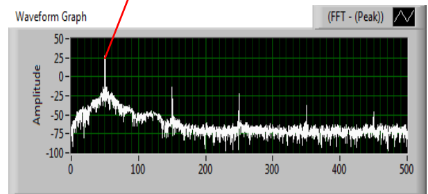
Fig 4: Healthy machine with Full load
