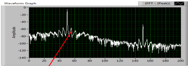
Fig 14: Winding Fault machine (50% winding faulted)
