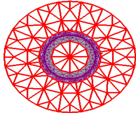
Fig 2: Mesh diagram for Three Phase Induction Machine
