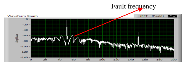
Fig 13: Winding Fault machine (20% winding faulted)
