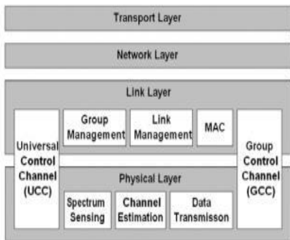
Fig. 3: General ISO/OSI Model for Cognitive Radio [24]
