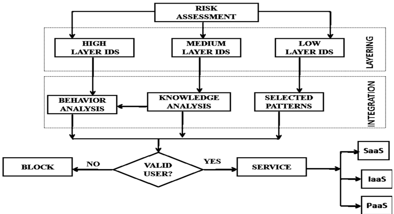
Figure 1: Risk assessment using Layered IDS
