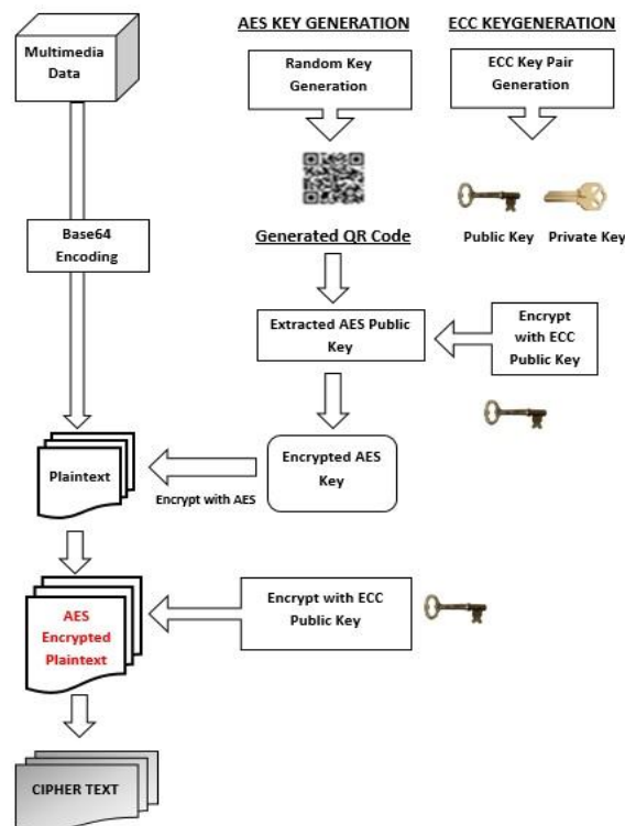
Fig 3. Encryption Process
