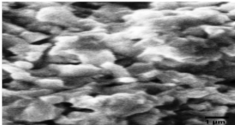
Fig.2. Scanning electron micrographs of BiFeO 3 ceramics
