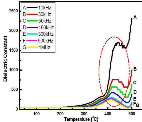
Fig.3. Dielectric constant versus temperature measurement in the frequency range 10 kHz–1 MHz for BiFeO 3 (curves A–G) sample
