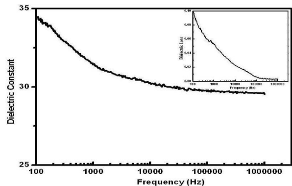
Fig.4. Dielectric constant and loss versus frequency measurement at RT of BiFeO 3
