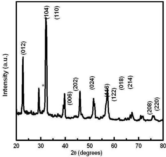
Fig.1. X-ray diffraction (XRD) spectra of BiFeO 3 sintered at 725°C for 30 min. obtained by solid state reaction method
