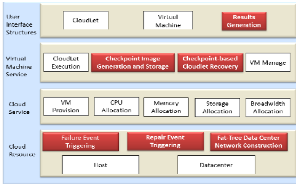
Fig 4: FTCloudSim Framework[9]
