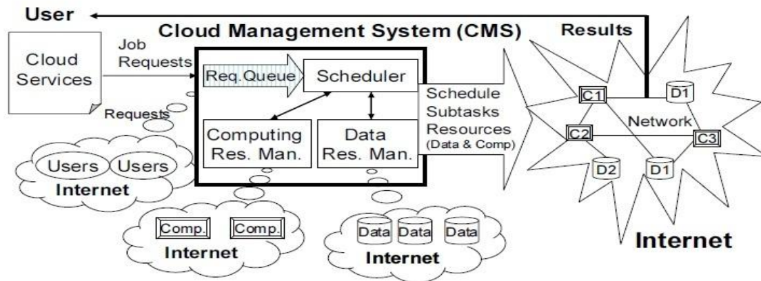
Fig 3: Cloud Service System[6]
