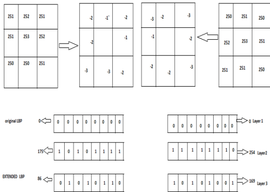
Fig: An example of Extended LBP Operator
