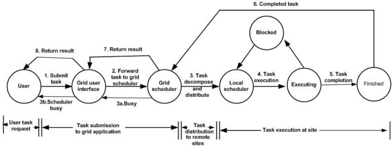
Fig. 5 Task States in Grid Computing
